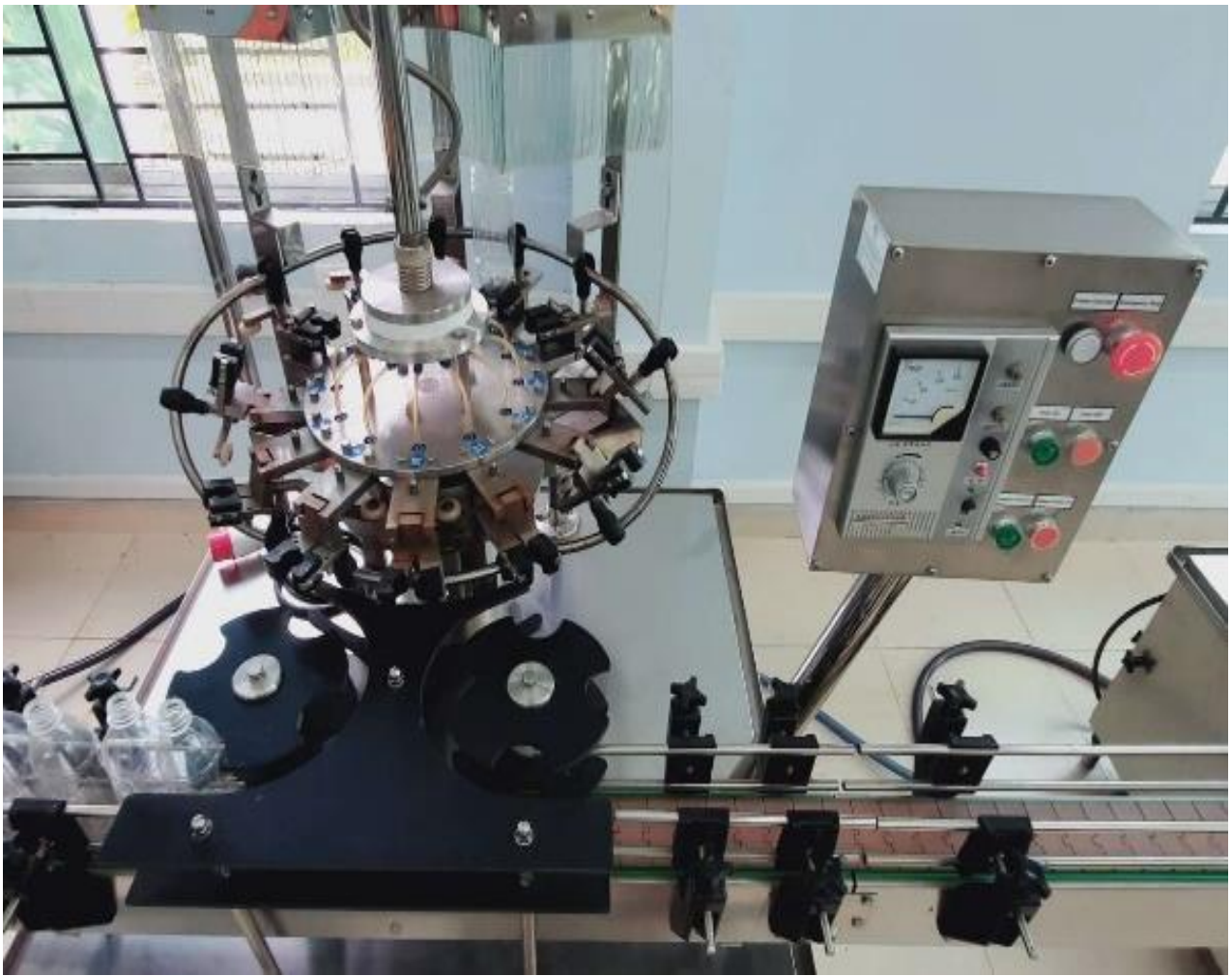
Figure 161: Cleaning station
