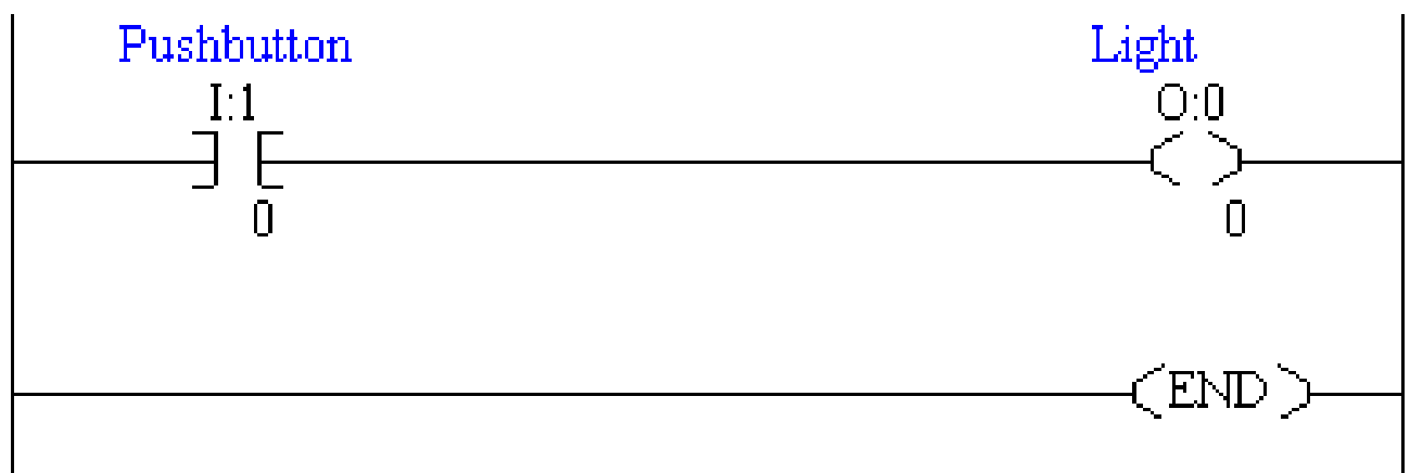
Figure 28: Ladder logic/diagram
