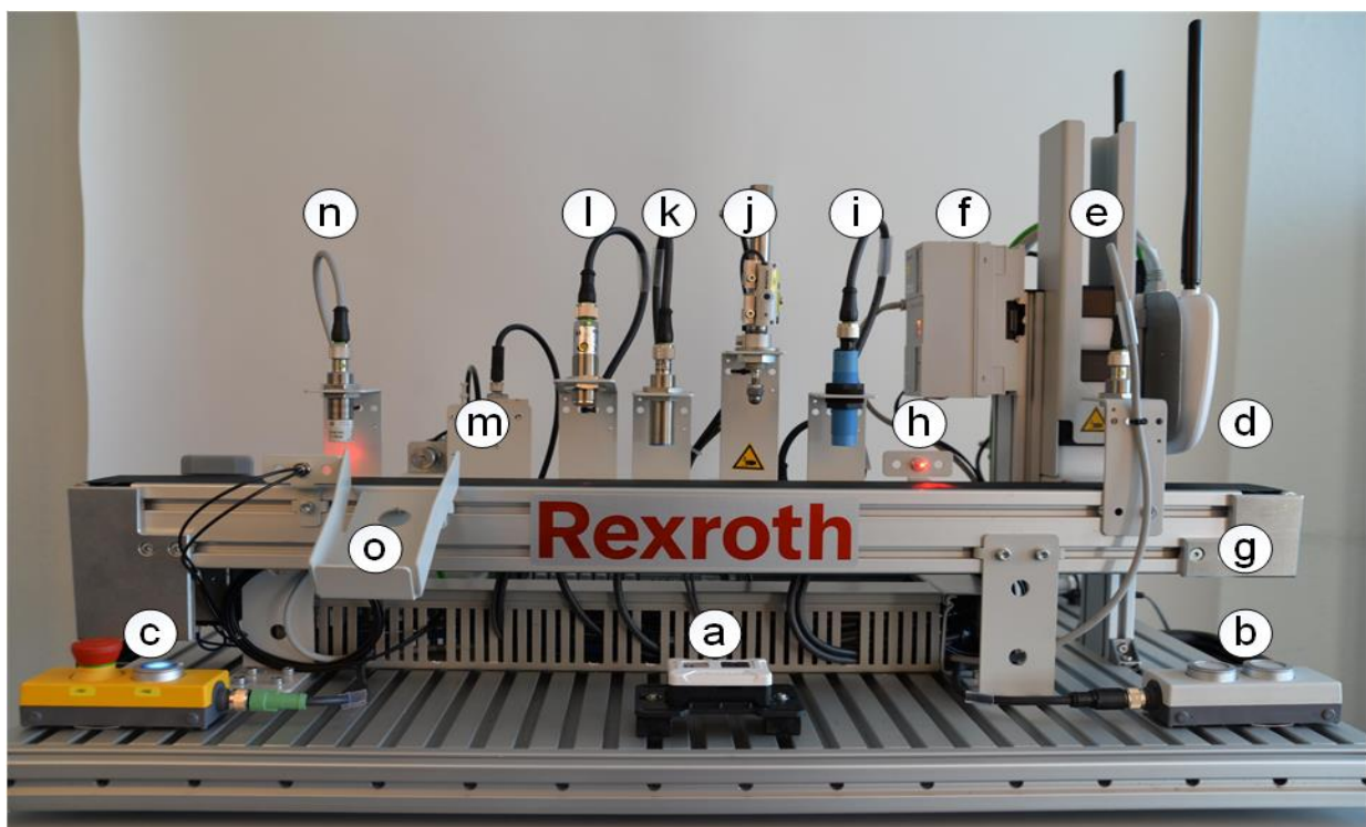
Figure 52: CPS i4.0 training system (front view)
