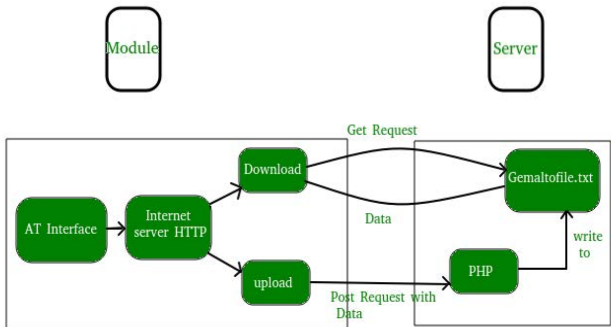
Figure 47: Webbased communication
